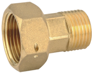
Brass Pipe Fitting Compression Female Connector
